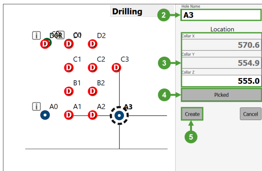
Figure 7-15 The operation sequence for creating an add hoc hole
